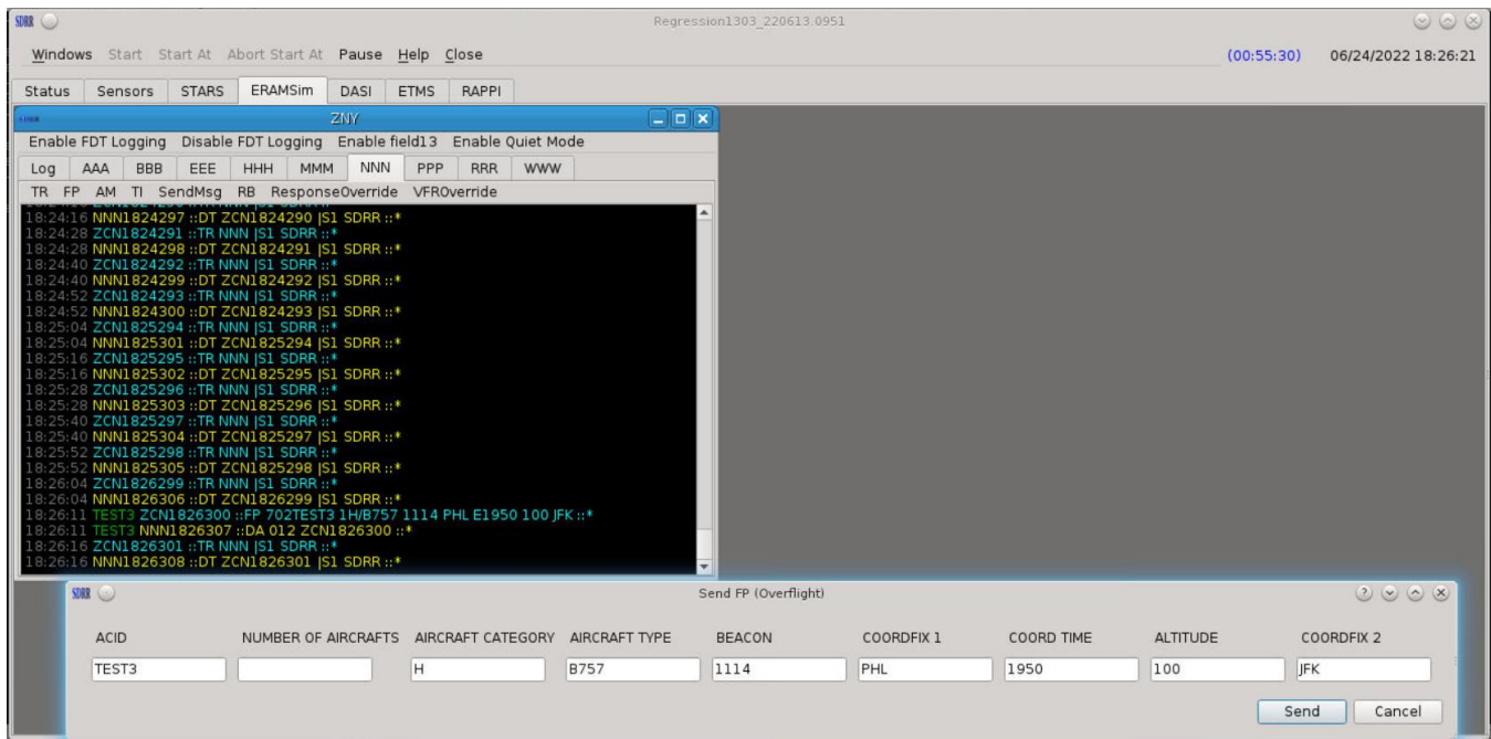
Figure 30. Send Flight Plan Example
