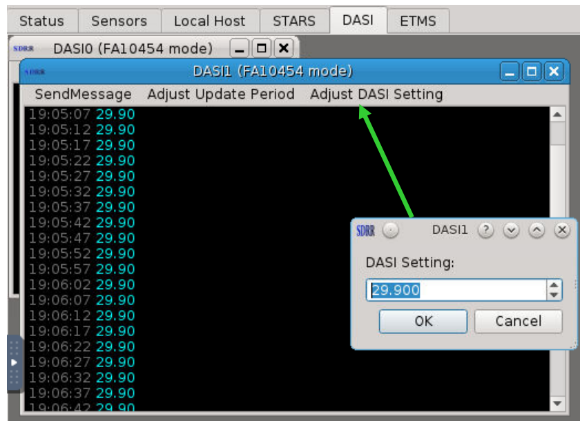
Figure 46. DASI Tab (Adjust DASI Setting)
