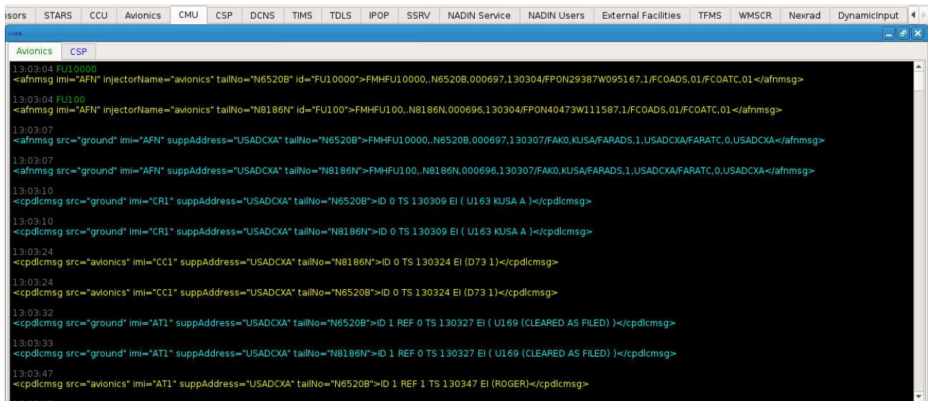
Figure 55. CMU Tab - Avionics
