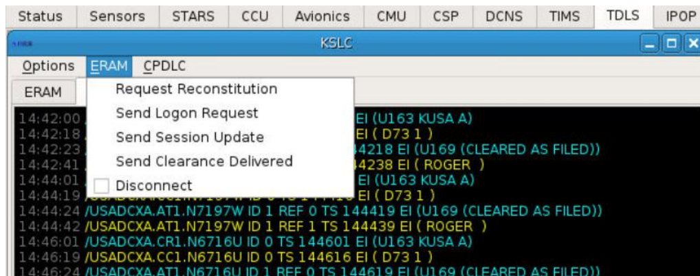
Figure 70. ERAM Session Selections
