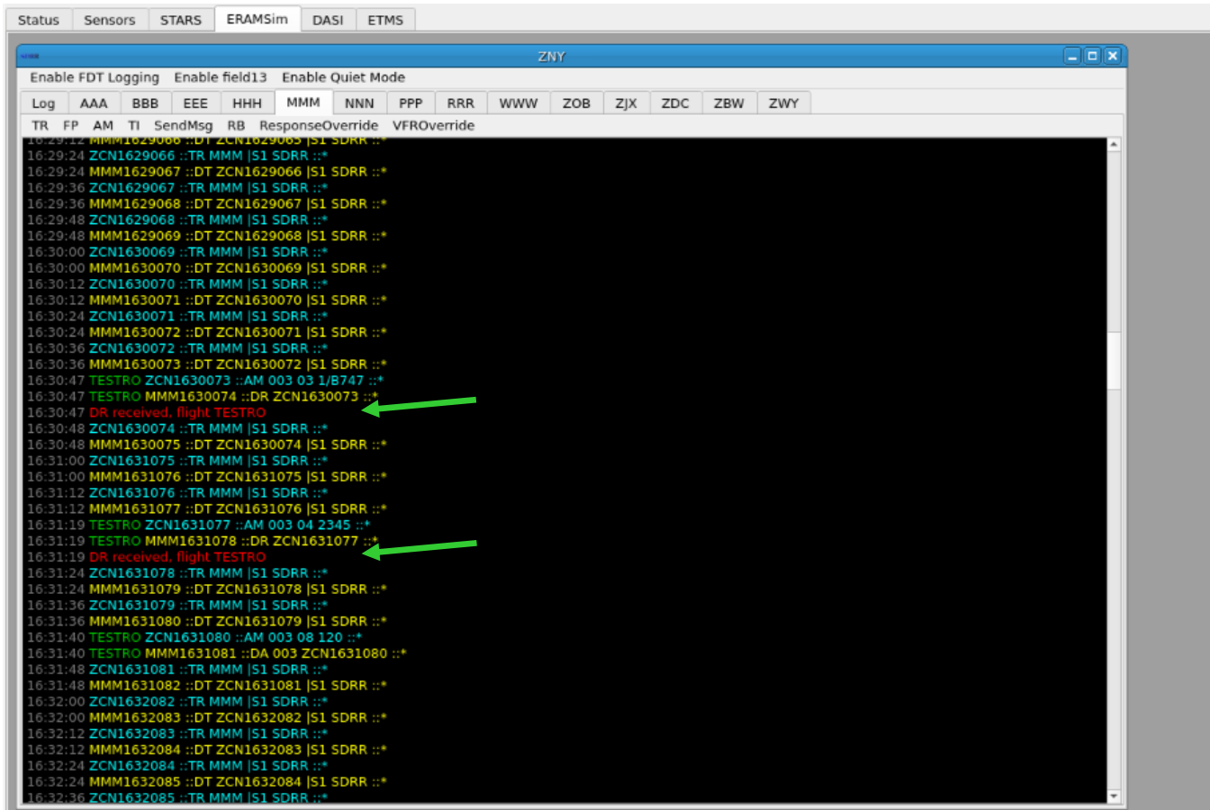
Figure 40. DRs from MMM for Flight TESTRO in ERAMSim Tab
