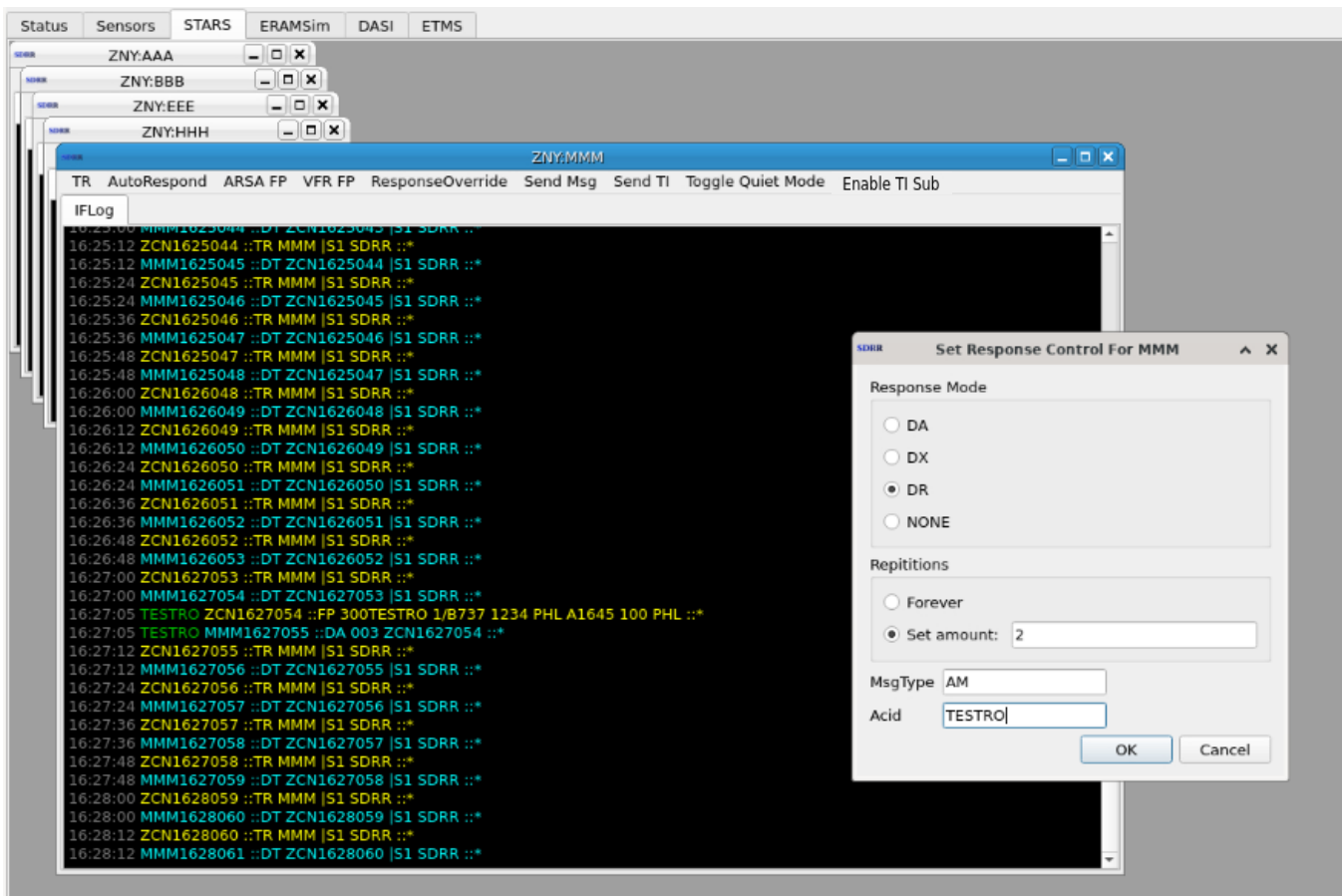
Figure 38. Response Override for MMM
