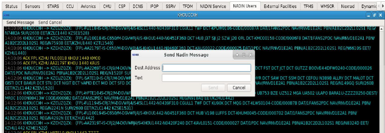
Figure 81. Send NADIN Message
