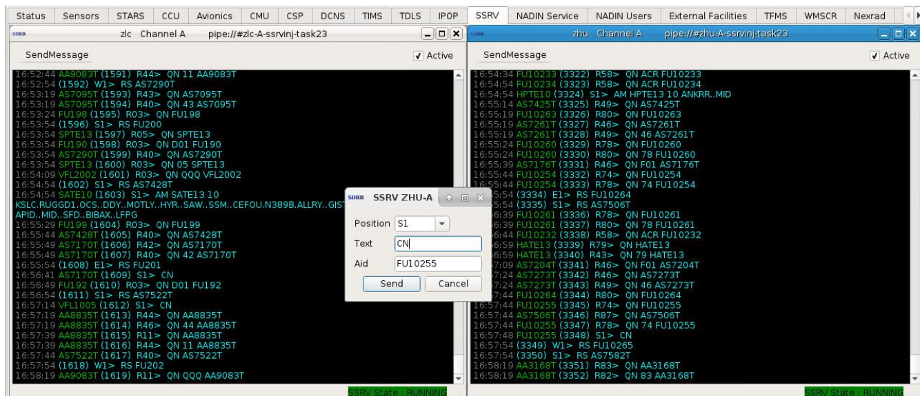
Figure 75. Send ERAM Message
