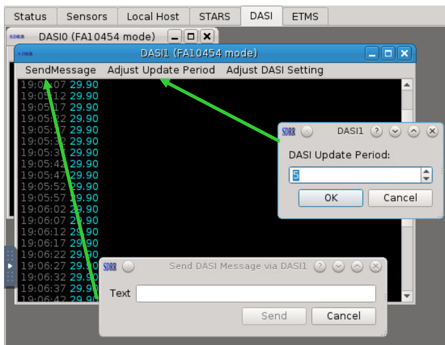
Figure 45. DASI Tab (SendMessage and Adjust Update Period)
