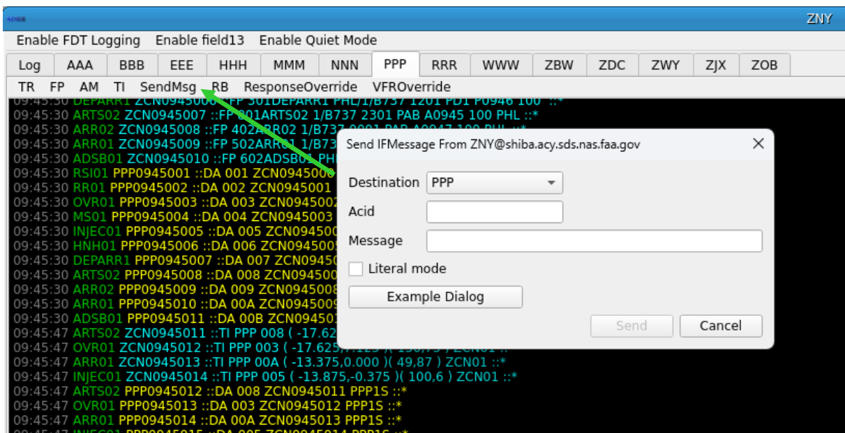
Figure 25. Send Interfacility Message
