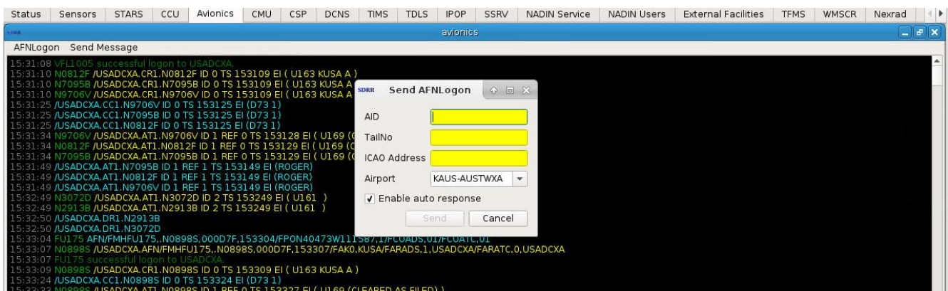
Figure 53. Send AFN Logon
