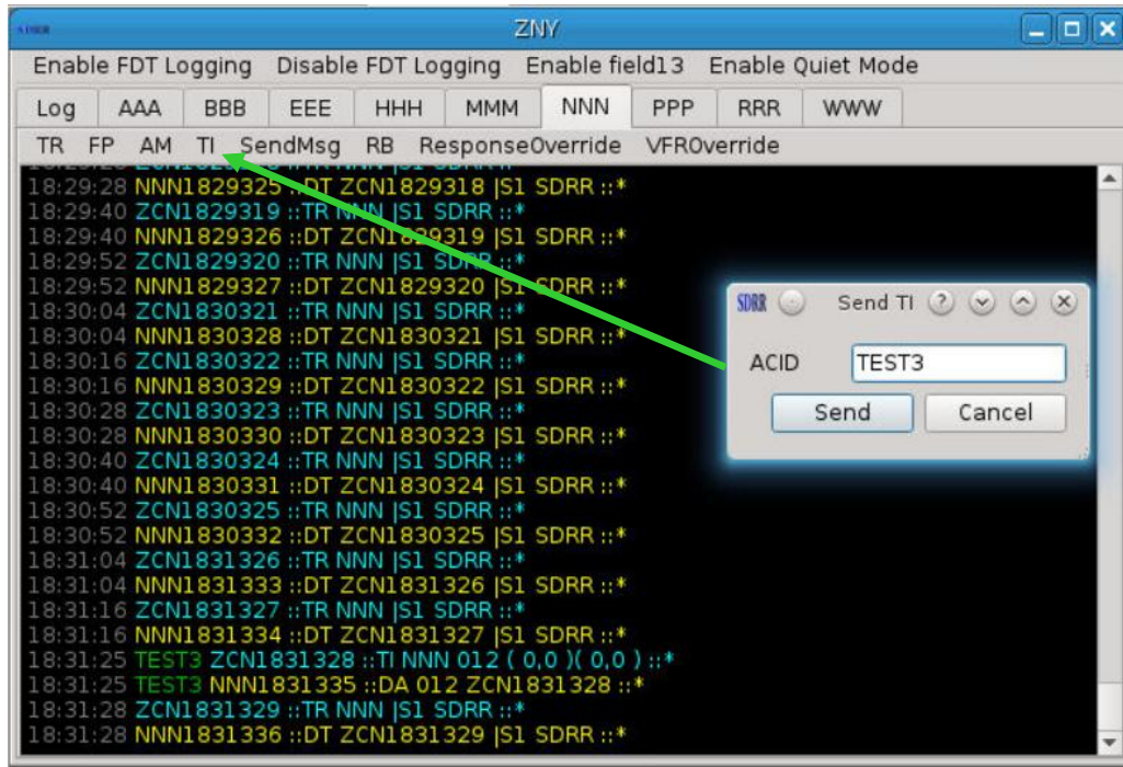
Figure 32. Send Transfer Initiate
