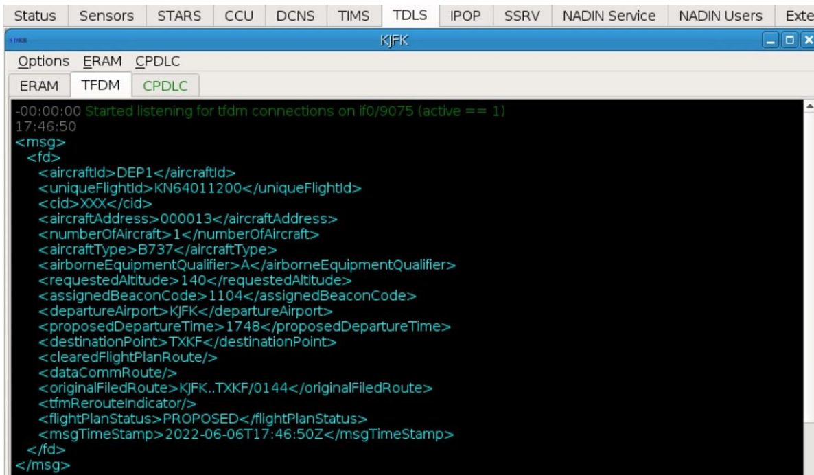
Figure 67. TDLS Tab - TFDM
