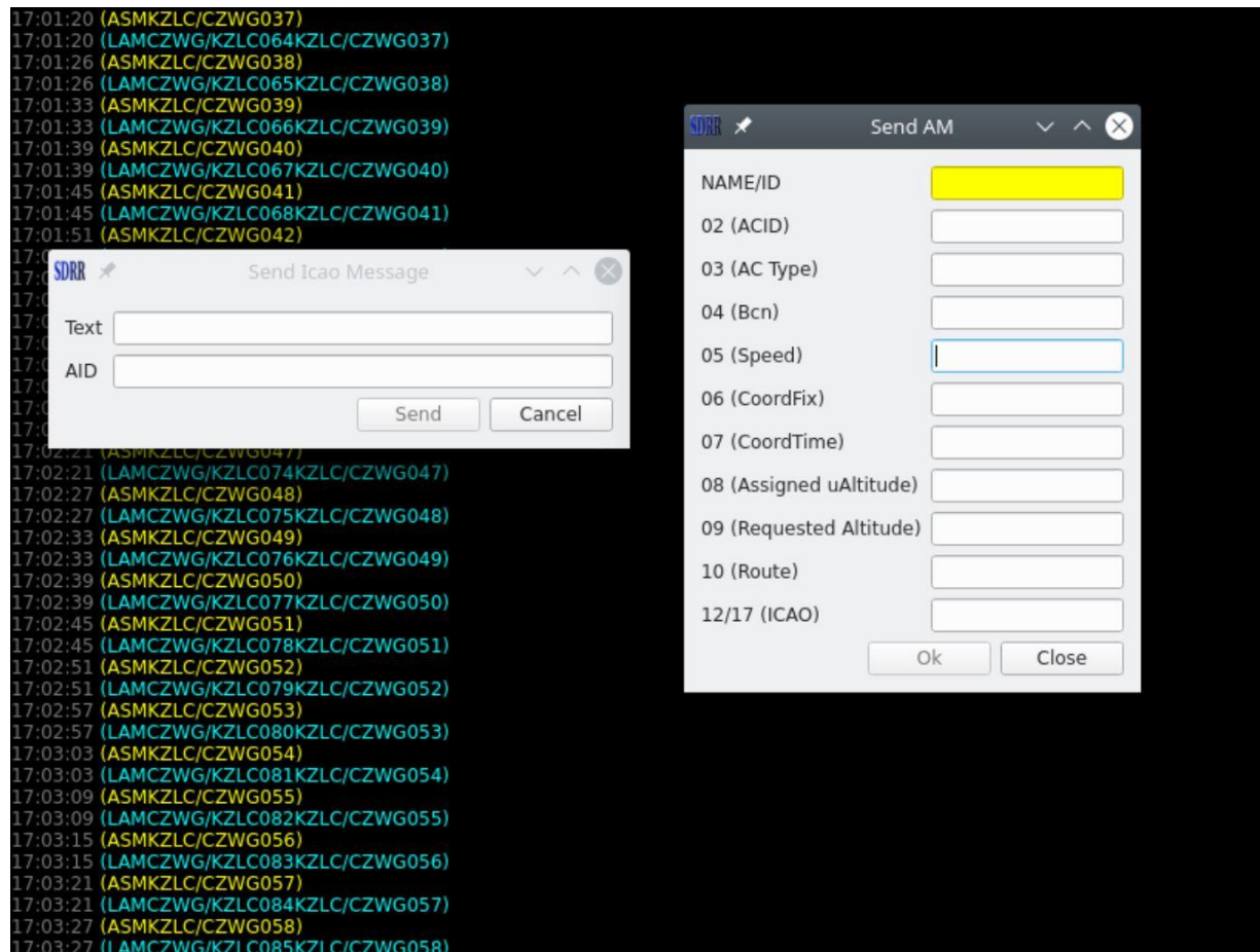
Figure 83. Send Message Dialog – Non US
