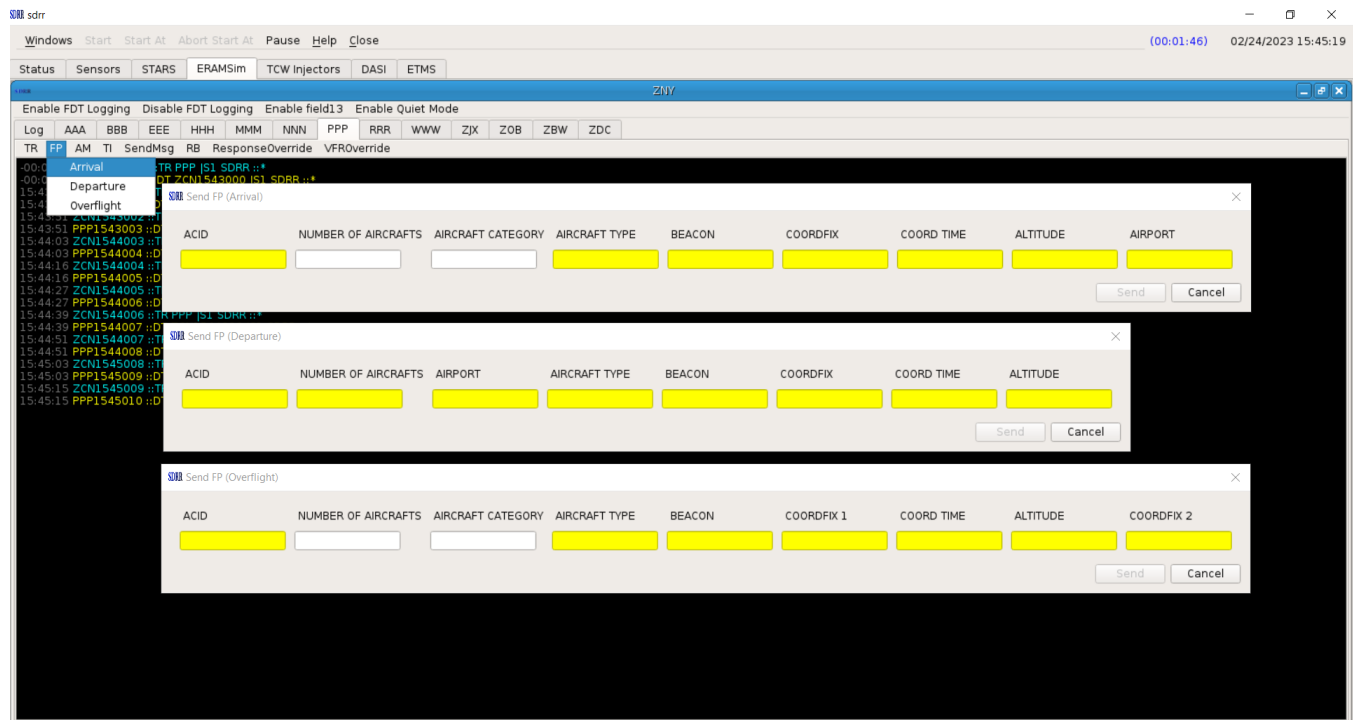
Figure 29. Send Flight Plan Types
