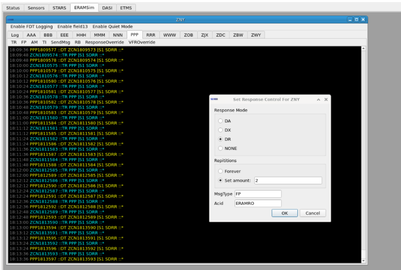
Figure 33. Response Override for ZNY
