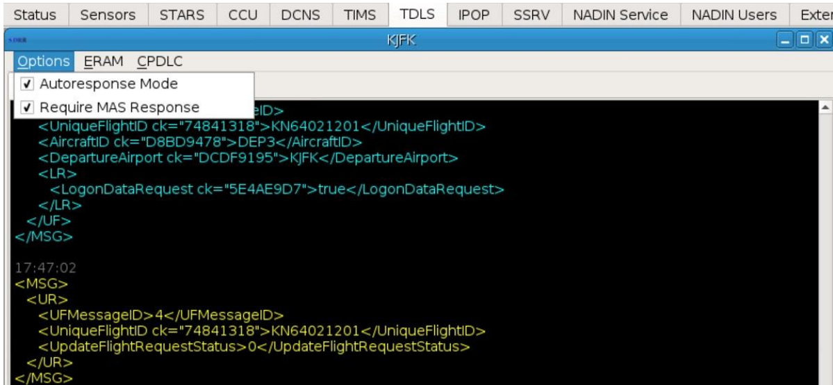
Figure 69. Autoreponse Mode & Require MAS Response Options
