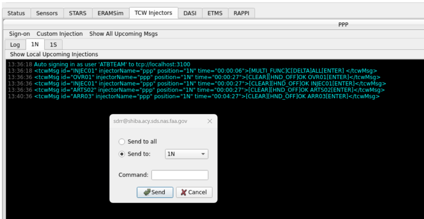
Figure 43. Custom TCW Injection
