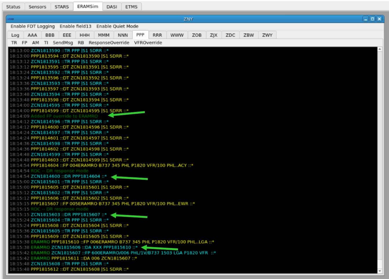
Figure 34. Response Override for ERAMRO in ERAMSim Tab
